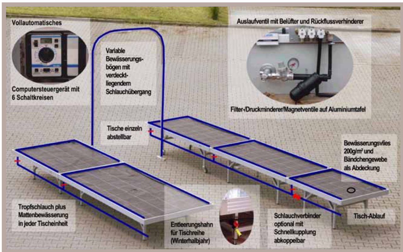
“Water Magic” automated irrigation system for benches and hanging baskets
